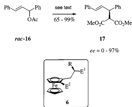
Scheme 7. Pd-catalyzed allylic alkylation; reaction conditions: x mol-% [Pd( \eta^3\text{-C}_3\text{H}_5 )Cl] 2 , y mol-% 6 , 1.0 mol-% KOAc, 3.0 equiv. dimethyl malonate/BSA, CH 2 Cl 2 , -20 °C or room temp.
