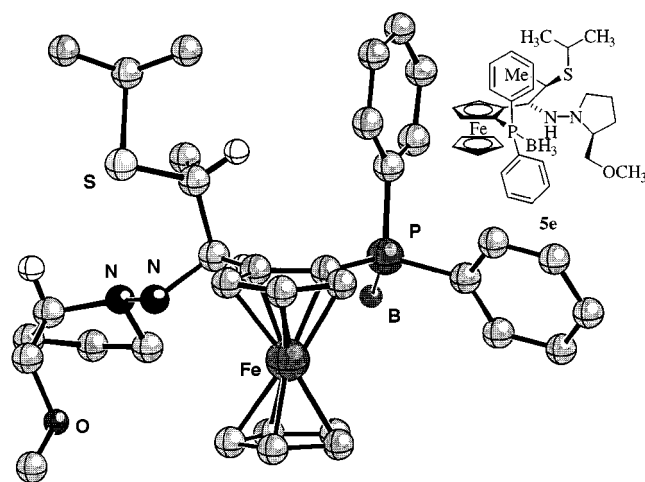
Figure 1. Crystal structure of hydrazine 5e
