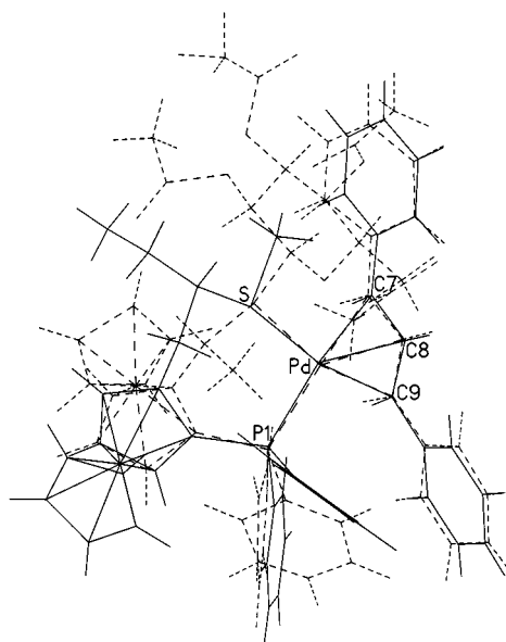
Figure 5. Schematic superposition of 20 (smooth line) and 21 (dotted line)
