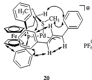
Figure 2. NOE connectivities for Pd complex 20
