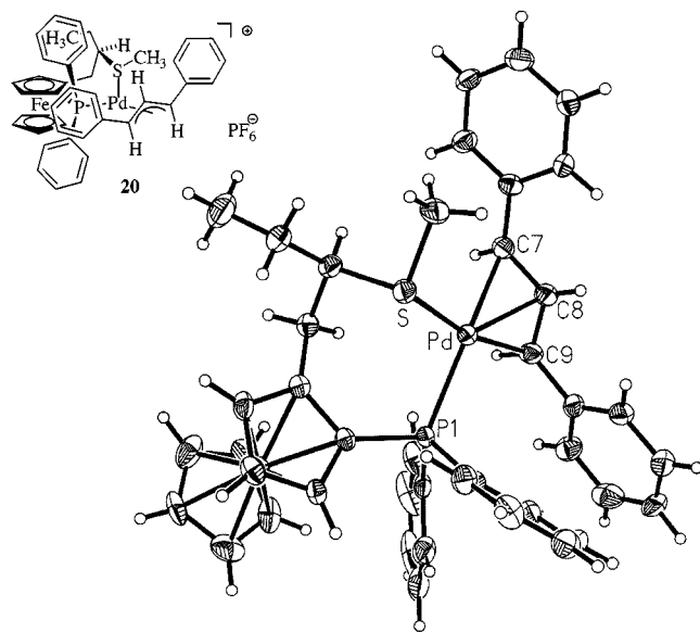
Figure 3. Crystal structure of Pd complex 20 (without anion and solvent) with 50% probability displacement ellipsoids; selected bond lengths are: Pd–S = 2.400(1), Pd–P1 = 2.326(1), Pd–C7 = 2.274(5), Pd–C8 = 2.188(4), Pd–C9 = 2.176(4), C7–C8 = 1.384(6) and C8–C9 = 1.404(6) Å
