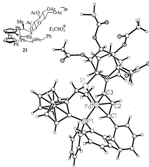
Figure 4. Crystal structure of the related Pd complex 21
