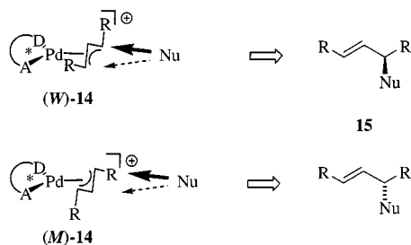
Scheme 6 D = \sigma -donor; A = \sigma -donor- \pi -acceptor
